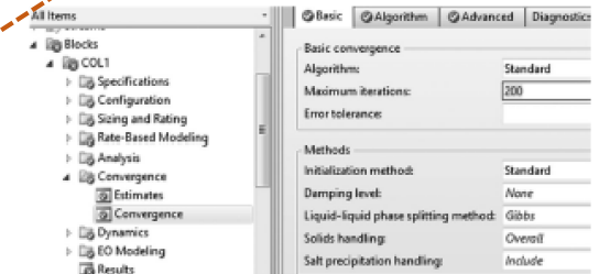
Figure 2.9 The Convergence form for the RadFrac block. Use this to change the maximum iterations and other parameters of the underlying numerical methods used to solve the model equations.
